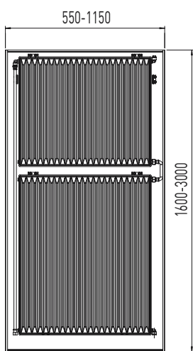
Height and length
