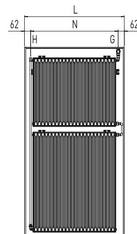
Built-in valve format 1 (top), rear view
