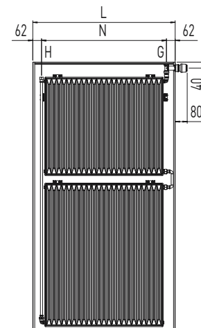
Built-in valve format 3 (top), rear view
